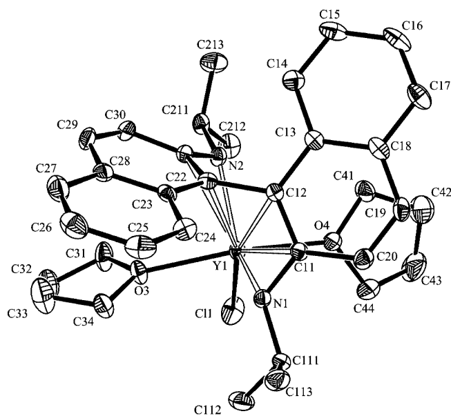
Figure 2. ORTEP drawing of complex 2 with the atom labeling scheme. Ellipsoids are drawn at the 30% probability level. The hydrogen atoms have been omitted for clarity. Selected bond lengths [Å] and angles [°]: \text{Y1--N1} 2.254(3), \text{Y1--N2} 2.257(4), \text{Y1--Cl1} 2.5835(14), \text{Y1--C11} 2.700(4), \text{Y1--C12} 2.756(4), \text{Y1--C21} 2.717(4), \text{Y1--C22} 2.746(4); \text{N1--Y1--N2} 123.36(15), \text{N1--Y1--Cl1} 115.78(12), \text{N2--Y1--Cl1} 120.86(10).
