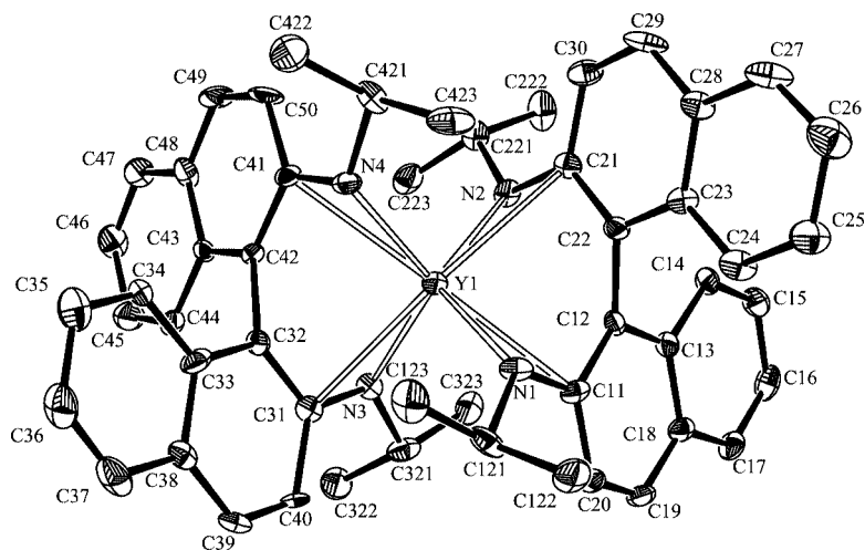
Figure 4. ORTEP drawing of complex 5 with the atom labeling scheme. Ellipsoids are drawn at the 30% probability level. The \text{Li}(\text{thf})_4^+ cation and the hydrogen atoms have been omitted for clarity. Selected bond lengths [ \text{\AA} ] and angles [ ^\circ ]: Y1–N1 2.297(5), Y1–N2 2.284(5), Y1–N3 2.290(5), Y1–N4 2.265(6), Y1–C11 2.712(6), Y1–C21 2.767(6), Y1–C31 2.733(7), Y1–C41 2.753(7); N1–Y1–N2 118.50(2), N1–Y1–N3 102.07(18), N2–Y1–N3 109.1(2), N1–Y1–N4 108.7(2), N2–Y1–N4 100.8(2), N3–Y1–N4 118.5(2).
