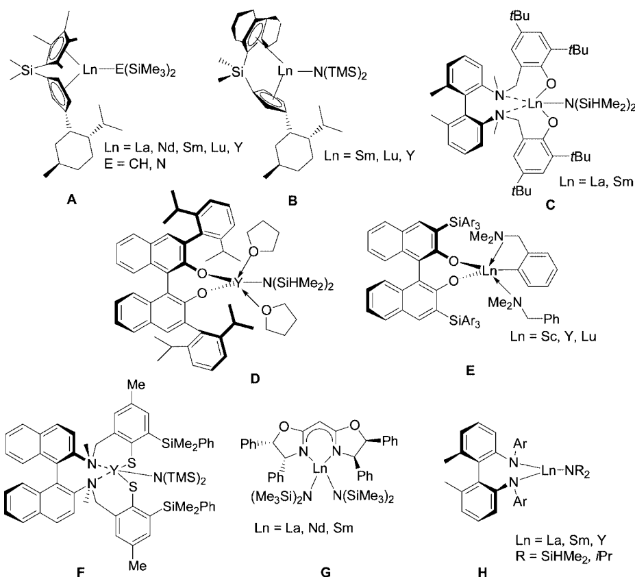
Figure 1. Complexes for intramolecular hydroamination reactions.
