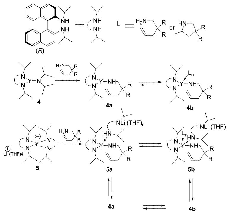
Scheme 6. Proposed structures for the intermediate catalytic species.
