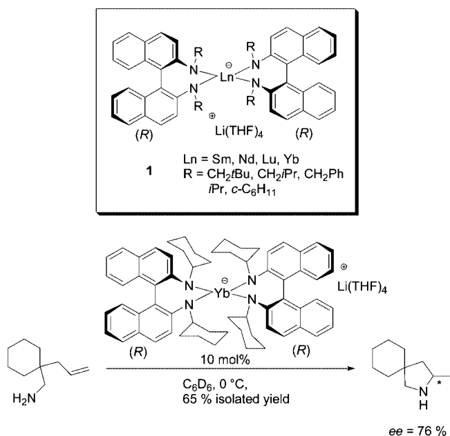
Scheme 1. Intramolecular hydroamination catalyzed by chiral lanthanide ate complexes.
