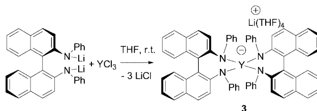
Scheme 3. Synthesis of the yttrium ate complex [\text{Li}(\text{thf})_4][\text{Y}\{(R)\text{-C}_{20}\text{H}_{12}(\text{NPh})_2\}_2] ( 3 ).
