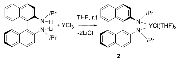
Scheme 2. Synthesis of the neutral yttrium complex [\text{Y}\{(R)\text{-C}_{20}\text{H}_{12}(\text{NiPr})_2\}\text{Cl}(\text{thf})_2] ( 2 ).
