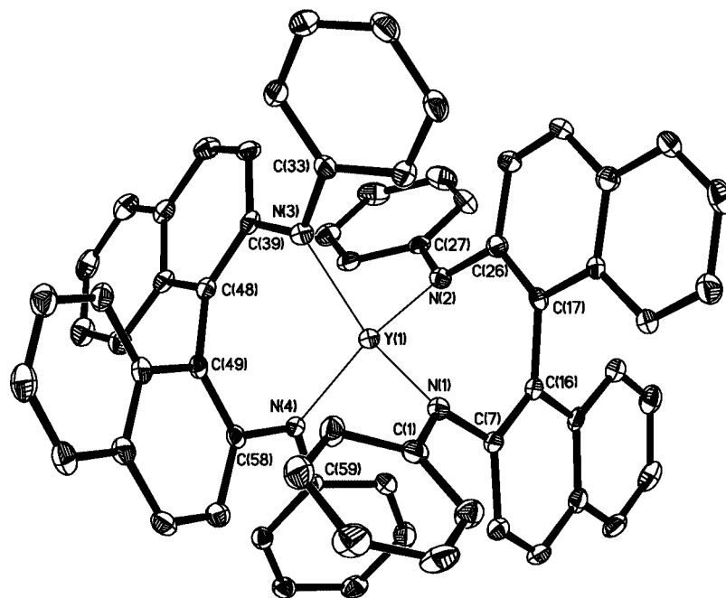
Figure 3. ORTEP drawing of complex 3 with the atom labeling scheme. Ellipsoids are drawn at the 30% probability level. The \text{Li}(\text{thf})_4^+ cation and the hydrogen atoms have been omitted for clarity. Selected bond lengths [ \text{\AA} ] and angles [ ^\circ ]: Y1–N1 2.275(2), Y1–N2 2.267(2), Y1–N3 2.270(2), Y1–N4 2.288(2), Y1–C26 2.747(2), Y1–C16 2.849(3), Y1–C7 2.727(3), Y1–C39 2.743(3), Y1–C58 2.746(3); N1–Y1–N2 118.47(8), N1–Y1–N3 103.74(8), N2–Y1–N3 104.69(9), N1–Y1–N4 108.65(8), N2–Y1–N4 103.84(8), N3–Y1–N4 118.15(8).
