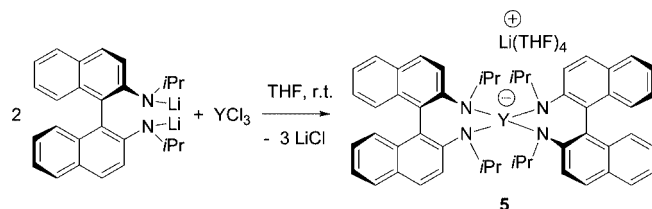
Scheme 5. Synthesis of the ate complex [\text{Li}(\text{thf})_4][Y\{(R)\text{-C}_{20}\text{H}_{12}(\text{N}i\text{Pr})_2\}_2] ( 5 ).
